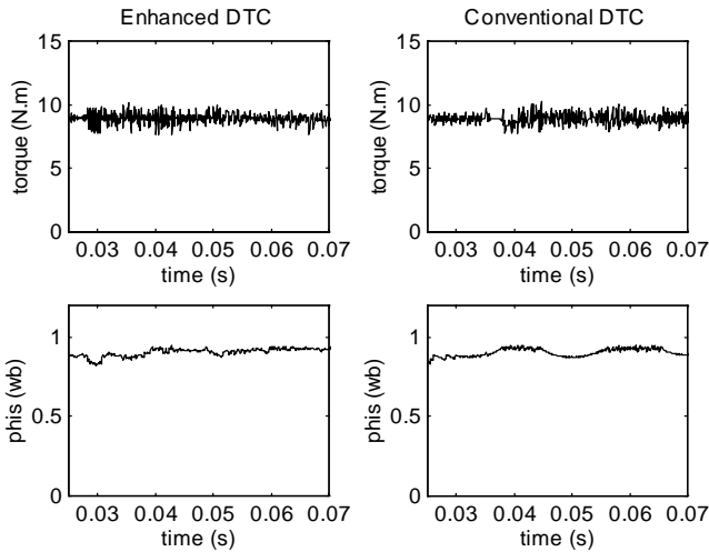
Fig. 8 : Torque response and flux
