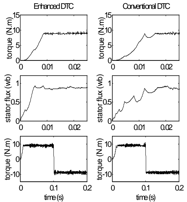
Fig. 6 : Torque and flux response
