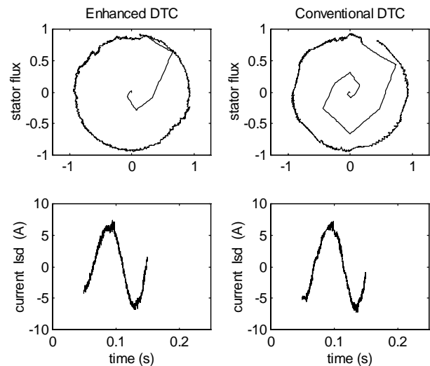
Fig. 7 : Vector flux locus and current response
