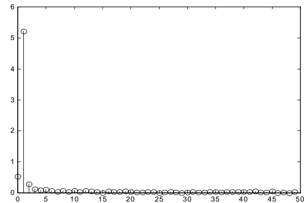
Fig. 5 : Current harmonics enhanced DTC
