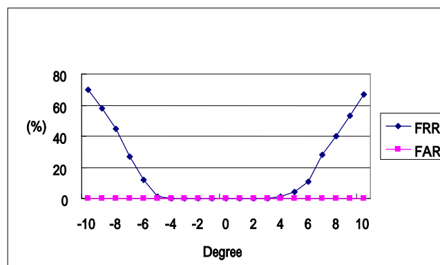
Fig.13 The effect of fingerprint rotation to the system
