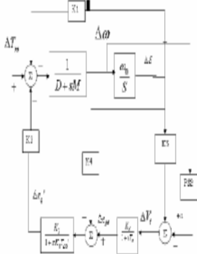
Fig.1 Linearized power system model model
