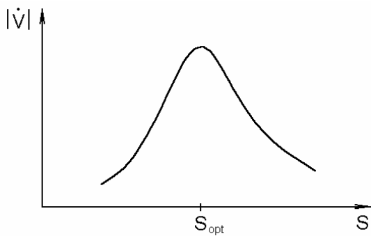
Fig. 4. Absolute value of Lyapunov function time derivative dependency on switch point S.
