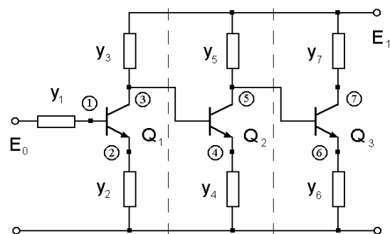
Fig. 2. Circuit topology for three-transistor cell amplifier.
