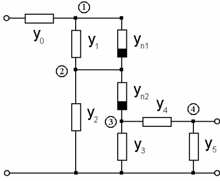
Fig. 3. Four-node circuit topology.
