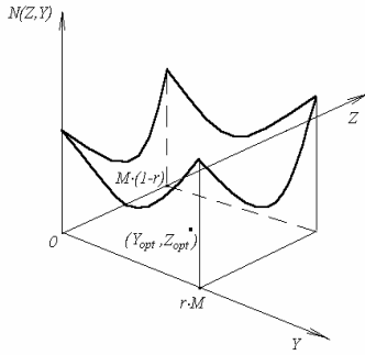
Fig. 1. Behavior of the function N(Y,Z) .
