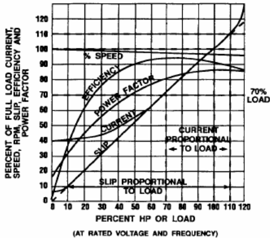
Fig2 -Typical NEMA Design B induction motor curve
