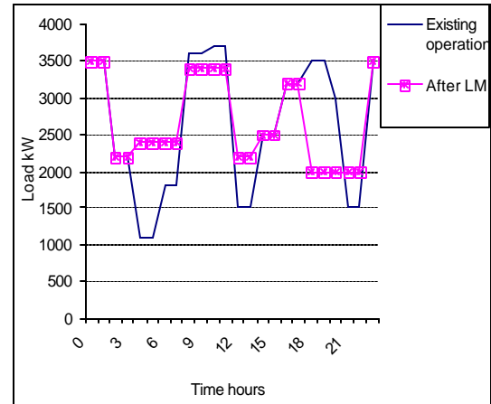
Fig. 2. Comparison of load curves under LM action
