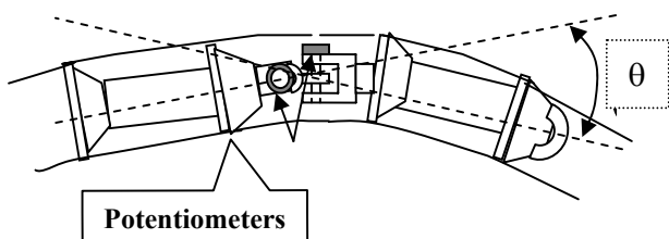
Fig. 2. Principle of angles measurement by means of potentiometers
