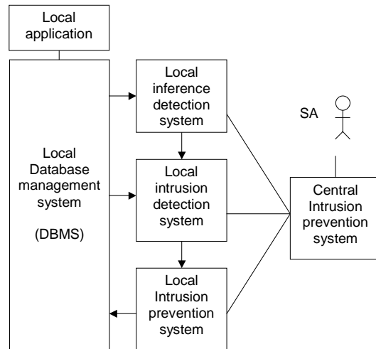
Fig. Intrusion Prevention System connected to a Database System.
