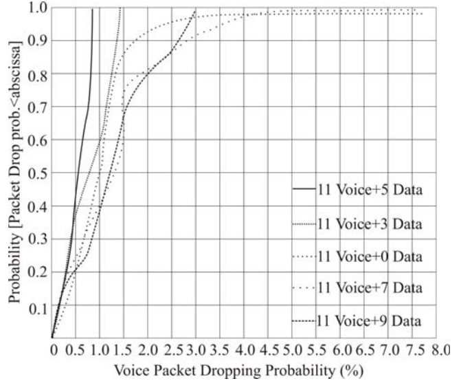
Fig. 1. CDF of Voice Packet Dropping Probability.
