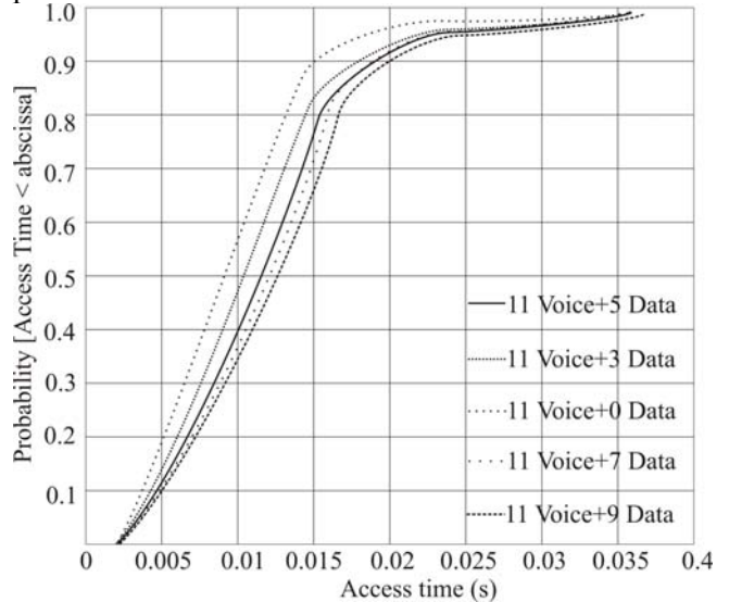
Fig. 2. CDF of average channel access time.
