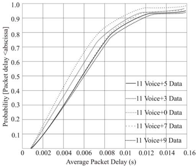
Fig. 3. CDF of average packet delay.
