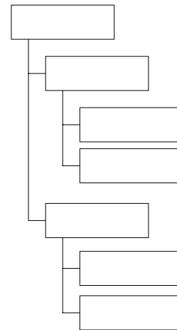
Fig. 1. Concept Hierarchy
