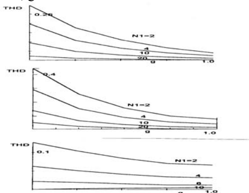
Fig.-4. Total harmonic distortion (THD) versus modulation factor g. (Top)-phase A, post-fault regime. (Middle)-phase B and C post-fault regime. (Bottom)-pre-fault regime
