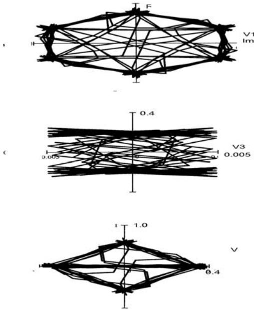
Fig.-3 Fourier approximation of voltage space vectors. Top: first symmetrical sequence. Middle : second symmetrical sequence. Bottom : Overall sequence.
