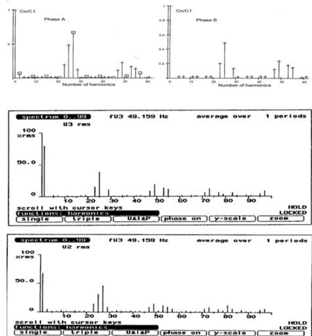
Fig.-5. Voltage harmonic spectrum .Analytical calculated (top trace). Experimental measured (middle trace) phase A ,(bottom trace) phase B and C.
