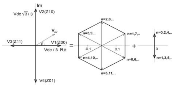
Fig.-2. Four voltage vectors (left) and their symmetrical components (right)
