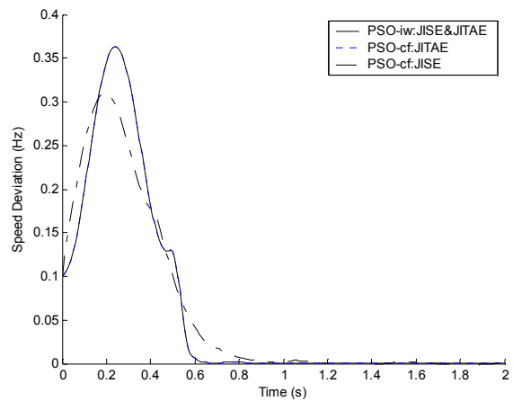
Fig. 2 Frequency deviation
