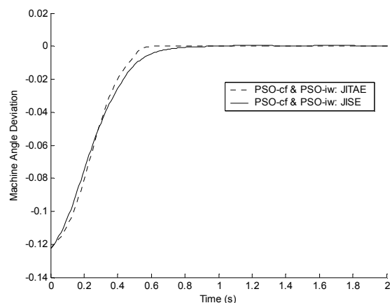
Fig. 3: Deviation of Machine's angle
