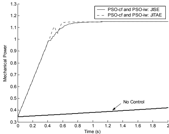
Fig. 4: Mechanical Power
