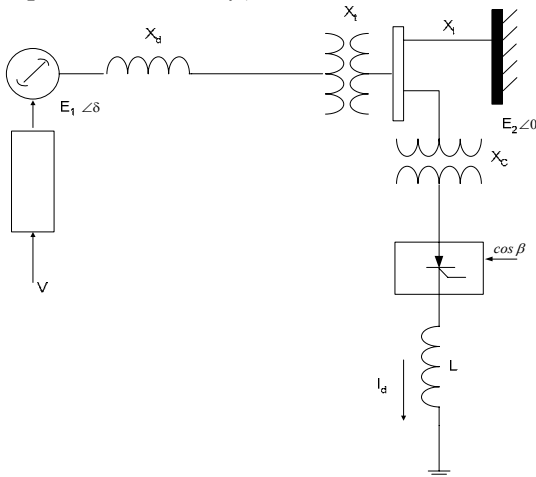
Fig.1 Nonlinear model of SMIB power system
