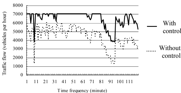
Fig. 2 Traffic flow compare with vs. without ramp metering control on freeway mainline
