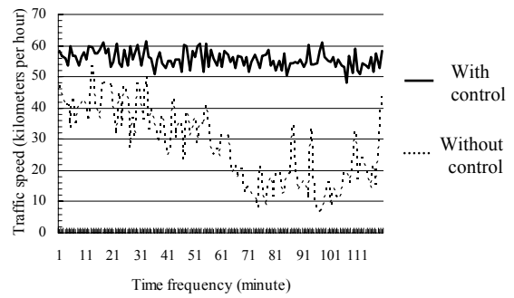
Fig. 3 Traffic speed compare with vs. without ramp metering control on C-D roadway
