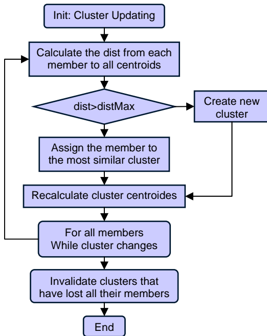
Figure 4. Description of the ‘k-means’ clustering algorithm
