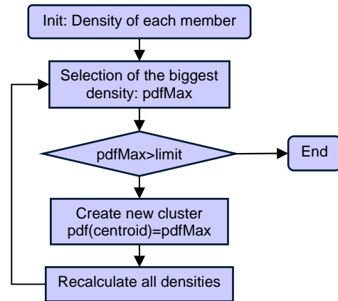
Figure 5. Description of the subtractive clustering algorithm
