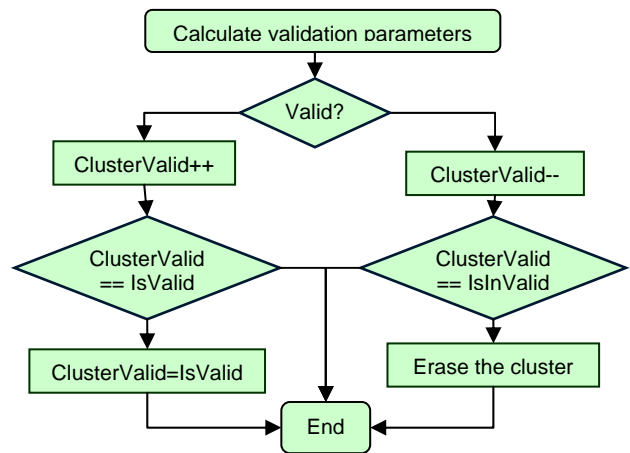
Figure 6. Description of the validation process for the clustering algorithm
