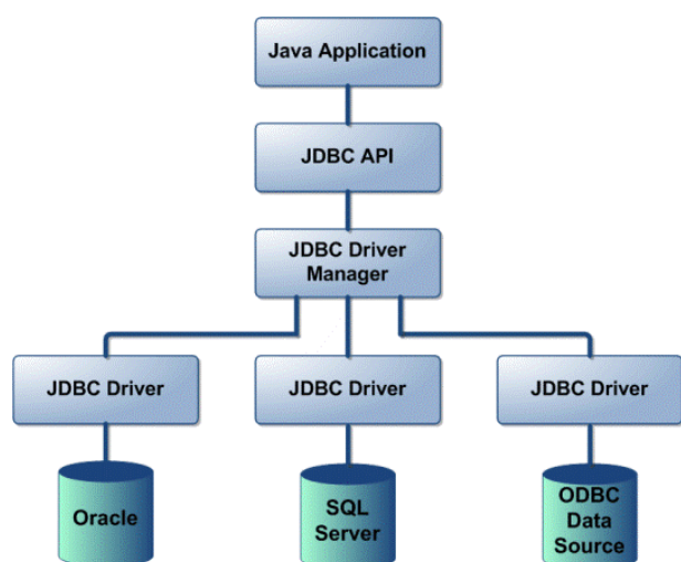
Figure 2. JDBC Architecture [4]
