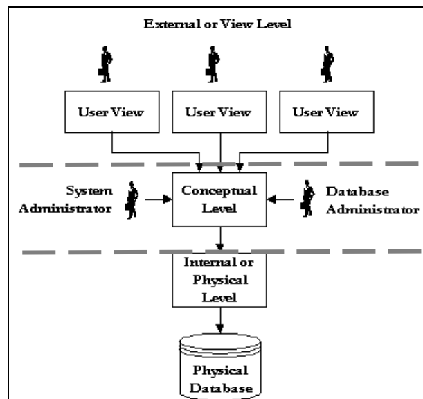
Figure 1. three level ANSI/SPARC architecture [13]
