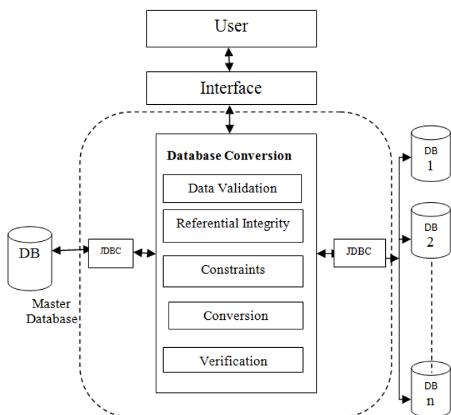
Figure 3. System architecture for flexible conversion
