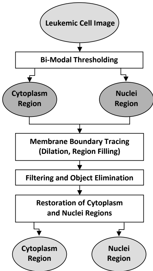
Fig 2. An overview of the segmentation process.
