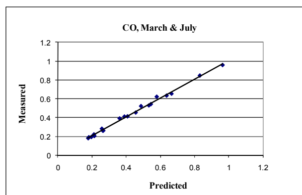
Fig.4: Measured and Predicted concentrations of CO during the period 6-12 March & July 2001, 2004, 2008
