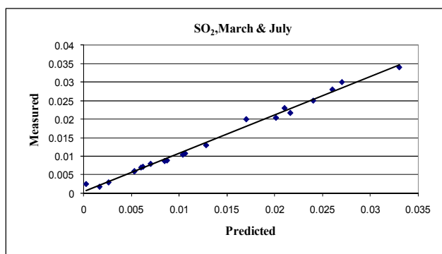
Fig.2: Measured and Predicted concentrations of \text{SO}_2 during the period 6-12 March & July, 2001, 2004, 2008
