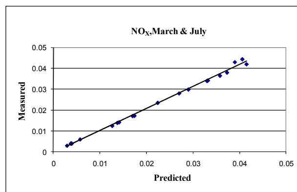
Fig.3: Measured and Predicted concentrations of \text{NO}_x during the period 6-12 March & July 2001, 2004, 2008
