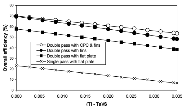
Fig. 19. Overall performance of PVT solar collector with single, double-pass system, double pass with compound parabolic solar collector and fins
