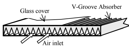
Fig. 3 The back-pass V-groove solar collector
