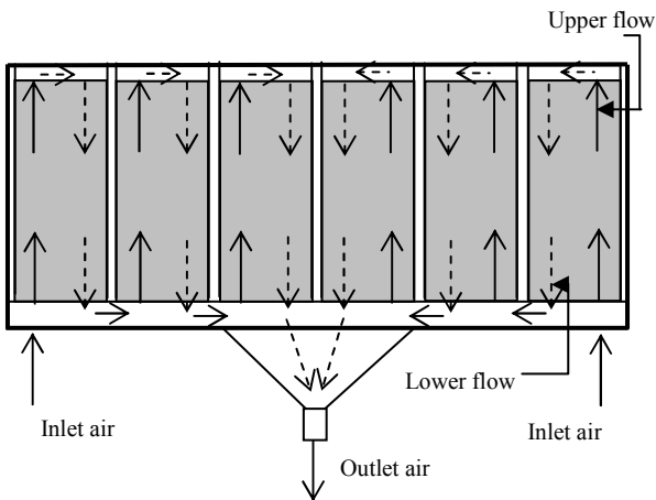
Fig.16. The collector arrangement for the solar dryer
