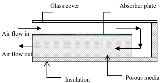
Fig.15. The schematic of a double-pass solar collector with porous media in the second channel
