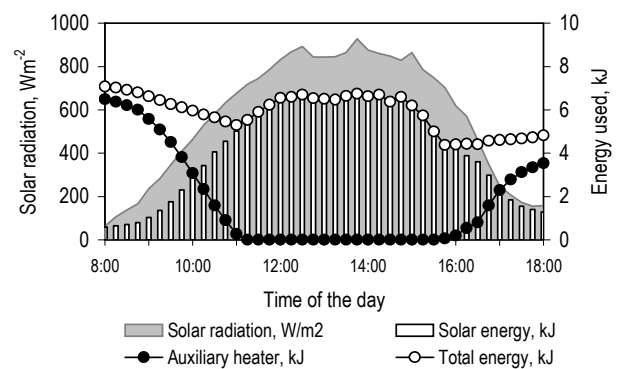
Fig. 4. Energy consumption during drying
