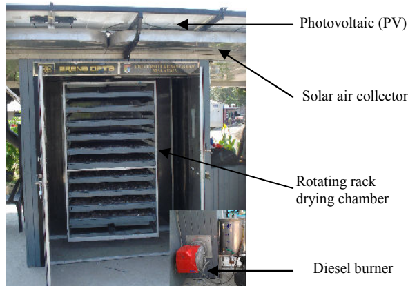
Fig.7. Photograph of salted silver jewfish in hybrid solar dryer with rotating rack chamber
