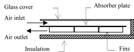
Fig. 11. The schematic of the solar dryer using double-pass solar collector with fins
