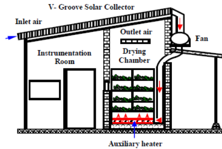
Fig. 1. The schematics of forced convection solar dryer with V-groove collector
