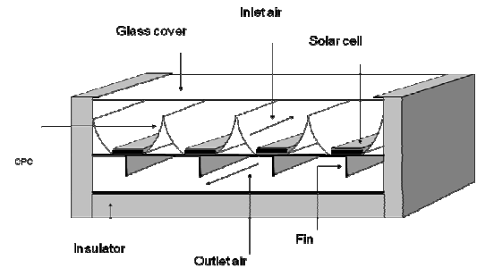
Fig. 17. The schematic of the solar dryer using double-pass solar collector with photovoltaic solar thermal collector
