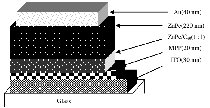
Fig. 3: Structure of the substrat/ITO/MPP/ZnPc/Au cell [23].
