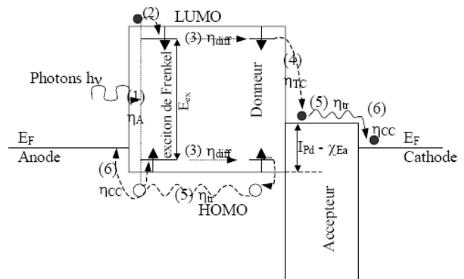
Fig. 2: mechanisms of the generation of carriers in an organic heterojunction [10].
