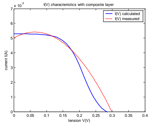
Fig. 10 : I(V) characteristic for the MPP/ZnPc structure contains the composite layer ZnPc/C 60 (1:1).
