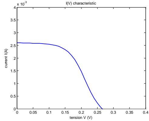
Fig.9: I(V) characteristic for the MPP/ZnPc structure.
