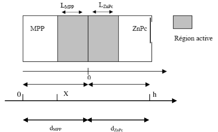
Fig. 4 : Geometrical model of the MPP/ZnPc structure [23].
