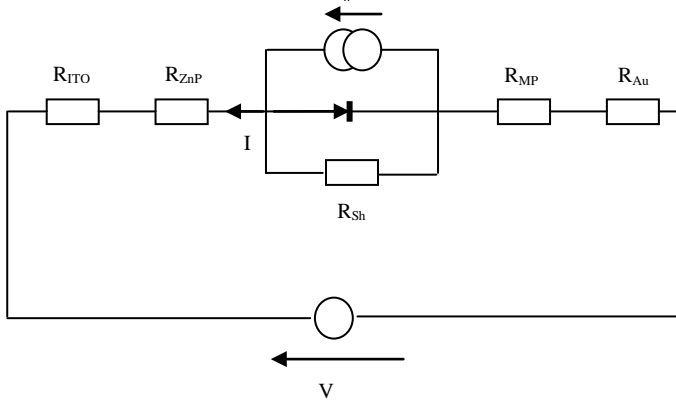
Fig. 8: Electric circuit of the MPP/ZnPc cell [23].
