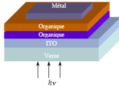
Fig. 1: Configuration of the structure of a double-layer photovoltaic cell [9].
