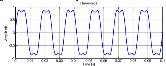
Fig. 1: Signals with Harmonics
