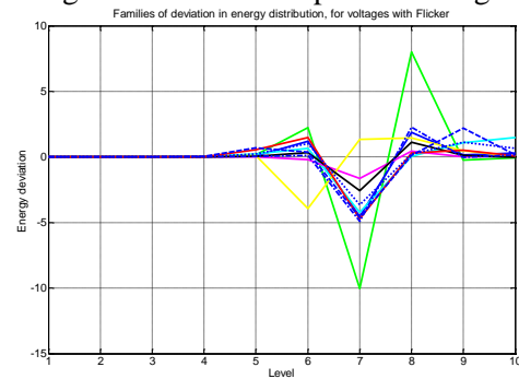
Fig. 8: Characteristic patterns – Flicker
