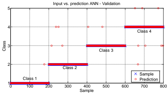
Fig. 10: Results MLP – Validation
