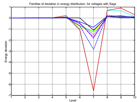
Fig. 7: Characteristic patterns - Sags
