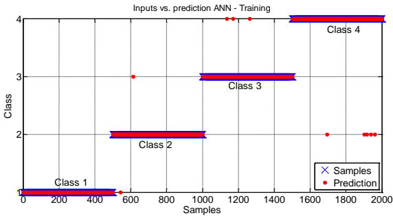
Fig. 9: Results MLP - Training
