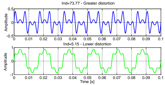
Fig. 16: Higher and lower harmonic distortion.
