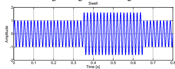
Fig. 3: Signals with Swell.
