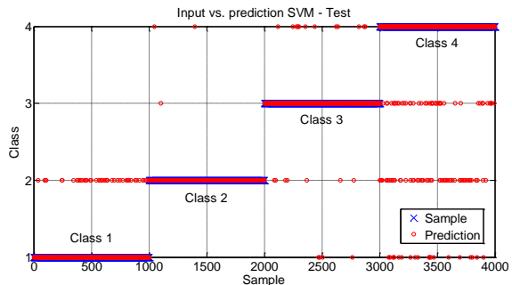
Fig. 14: SVM Results 1 – Test
