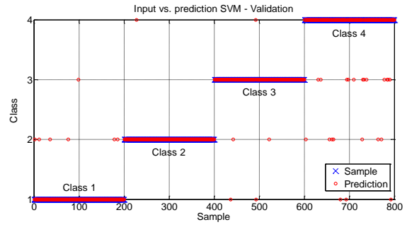
Fig. 13: SVM Results 1 – Validation
