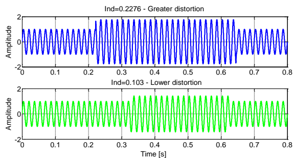
Fig. 18: greater than and less than– Swell
