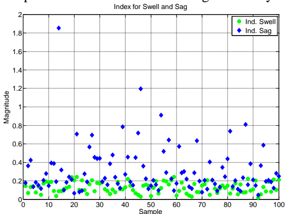
Fig. 21: Comparison Indicator - Swell and Sag
