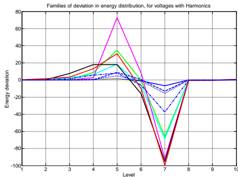
Fig. 5: Characteristic patterns – Harmonics
