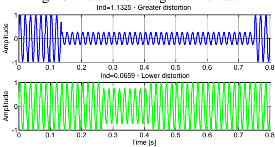
Fig. 20:- Greater and lower signals - Sag
