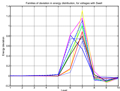
Fig. 6: Characteristic patterns – Swells
