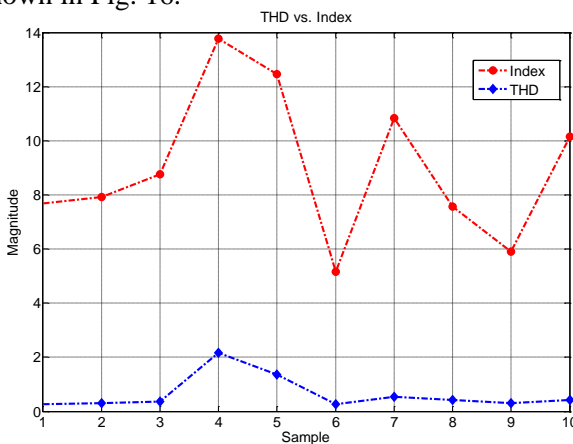
Fig. 15: Harmonic Parameters vs . Indicator
