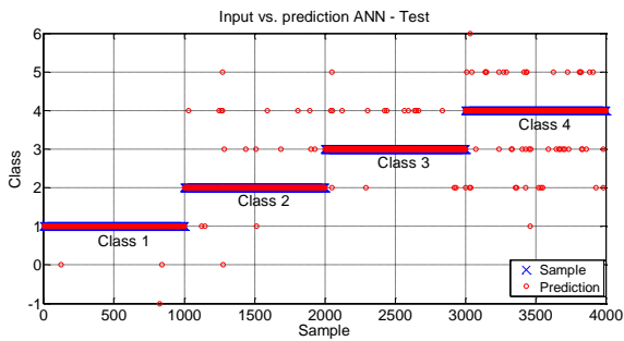
Fig. 11: Results MLP – Test.
