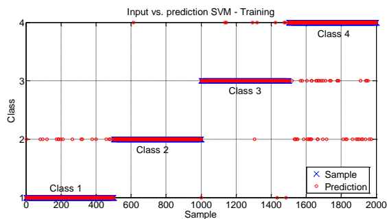
Fig. 12: SVM Results 1 - Training
