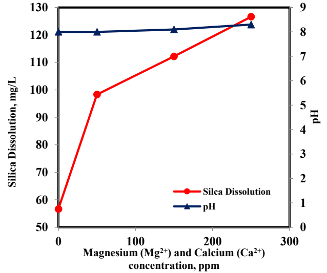
Fig.4: The effect of Mg 2+ and Ca 2+ ions on silica dissolution using crash core samples at 80°C
