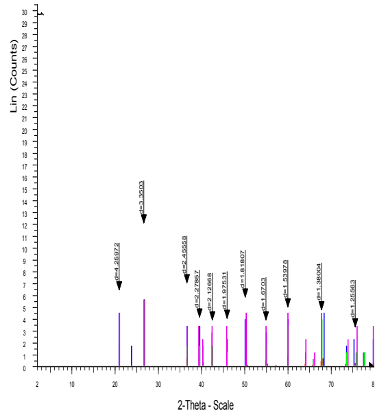
Fig.1: Core composition obtained from XRD
