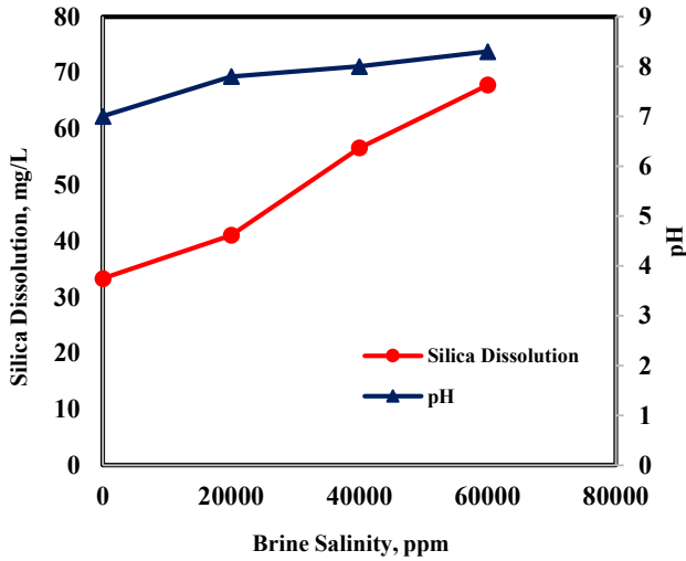
Fig.3: Brine salinity effect on silica solubility at 80°C
