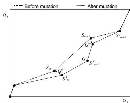
Figure 5: Structural mutation
