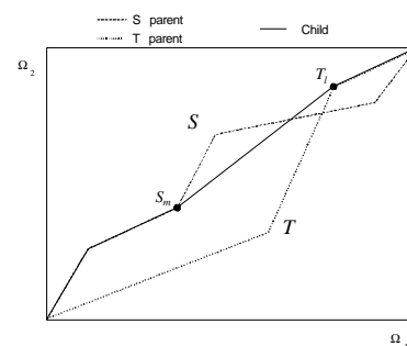
Figure 3. Crossover operator
