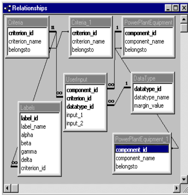
Fig. 1: Fuzzy Relational Database organization
