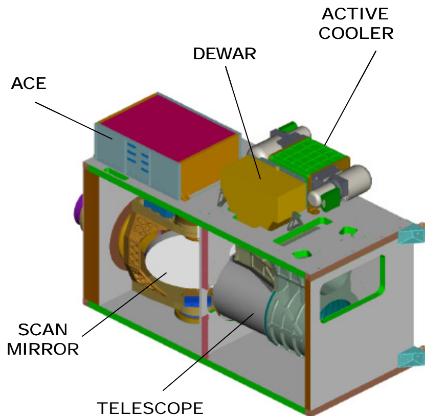
Figure 1. JAMI provides data with unprecedented detail and fidelity by means of recently proven new technology such as active cooling that was implemented successfully in a compact, efficient design architecture.
