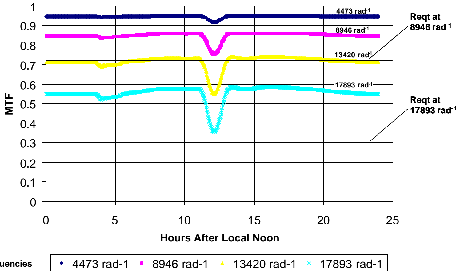
Figure 3. JAMI meets MTSAT-1R visible MTF requirements with margin even around local midnight for the worst case (shown here) of the Sun transiting across the south limb of the Earth.
