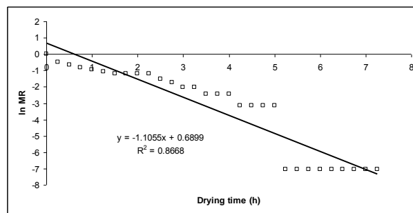
Fig. 8. Plot of \ln MR versus drying time (Henderson-Pabis model) at 30% RH
