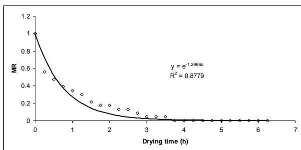
Fig. 6. Plot of MR versus drying time (Newton model) at 20% RH
