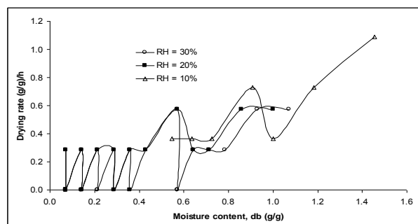
Fig. 5. Drying characteristic curves: dry basis moisture content versus drying time at 55°C and air velocity of 1 m/s
