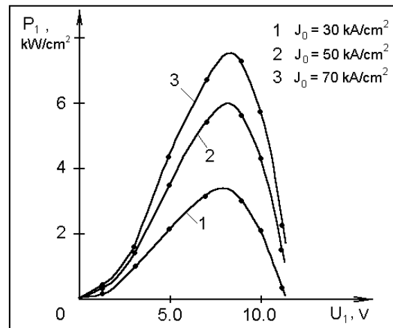
Figure 7. Output generated power P dependency as function of first harmonic amplitude U_1 for 220GHz.
