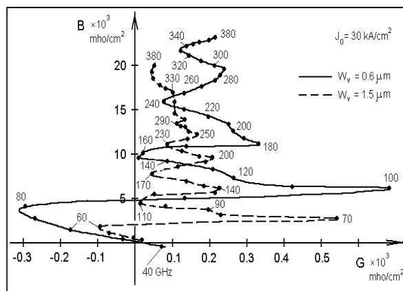
Figure 3. Complex small signal DAR diode admittance (conductance -G versus susceptance B ) for different frequencies and two values of drift layer widths W_v .
