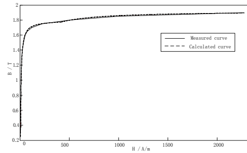
Fig.6 The magnetization curve of Measured and calculated
