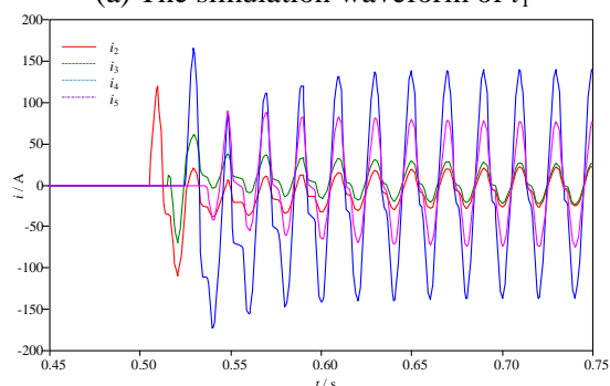
(b) The simulation waveform of each control winding current
