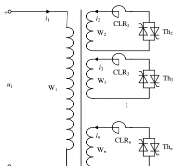
Fig.1 Basic circuit diagram of CRT
