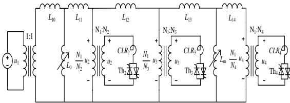
Fig.4 Circuit model of CRT
