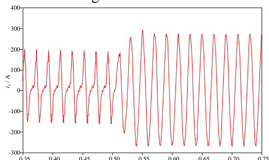
(a) The simulation waveform of i_1
