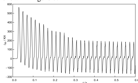
Fig.7 Excitation current of CRT
