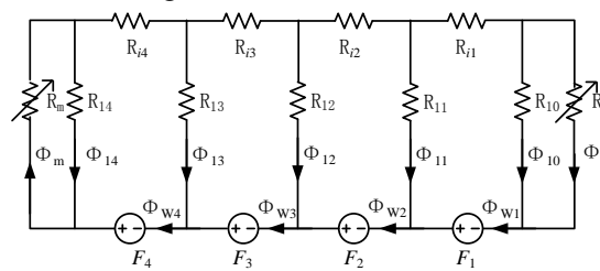
Fig.3 Magnetic circuit model of CRT
