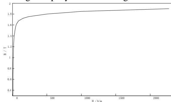
Fig.5 Magnetization curve of grain-oriented magnetic steel sheet
