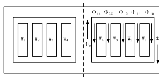
Fig.2 Core winding structure of CRT
