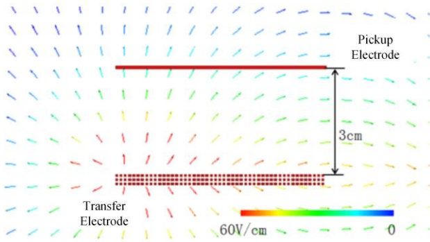
Fig.5. Electricfield distribution of meander-type coupled structure
