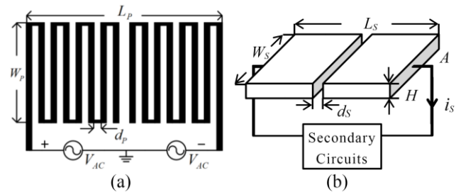
Fig. 4. Structure of meander-type transmitting and receiving electrodes
