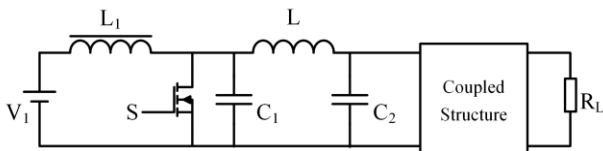
Fig.11. CCPT experiment equipment based E-class converter
