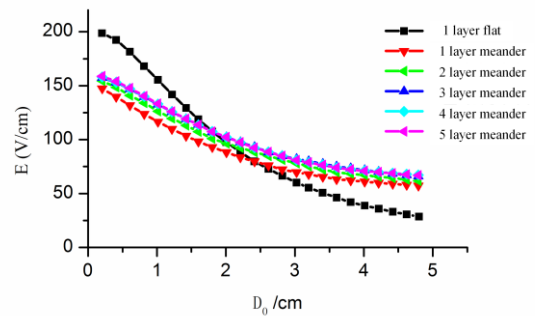
(a) Vertical electricfield distribution of meander electrodes
