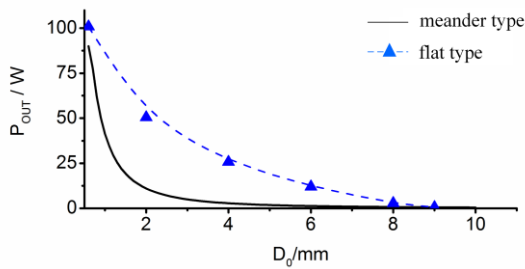
Fig.10. Transfer capability curves of meander-type CCPT system varying with D
