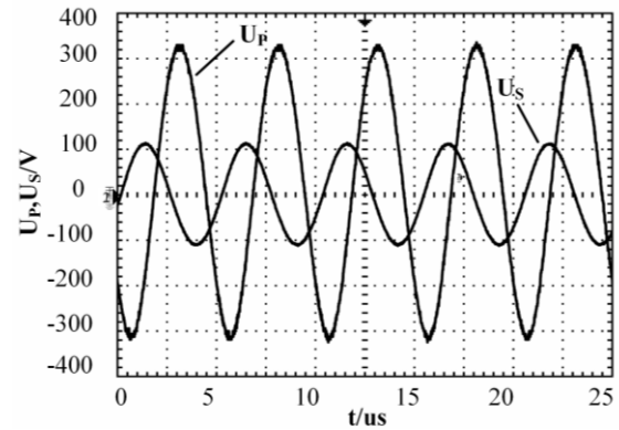
(a) Voltage waveform of transmitting and pickup electrodes
