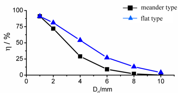
Fig.13. Comparison between transmission efficiency of meander-type CCPT system and flat-type
