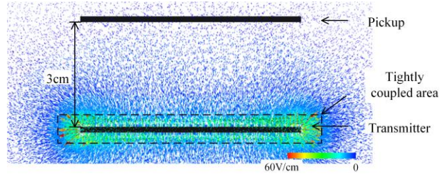
Fig.3. Electric field distribution of flat electrode loosely coupled
