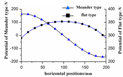
(b) Comparison between meander type and flat type electrodes
