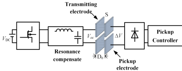
Fig.1. Schematic diagram of CCPT system based flat electrodes
