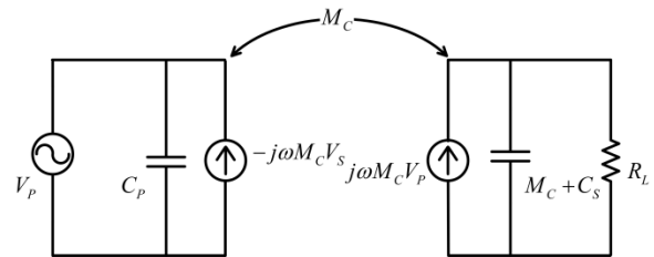
Fig.9. Equivalent circuit smodel of flat-type coupled structure
