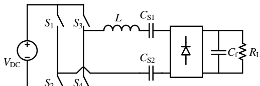
Fig.2. Topology of typical CCPT system based flat electrodes
