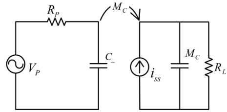
Fig.8. Equivalent circuit model of meander-type coupled structure
