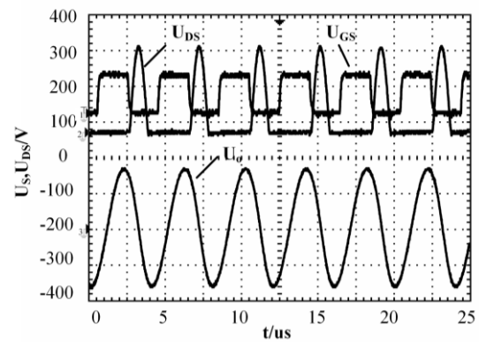
(b) Drive signal U_{GS} and output U_o
