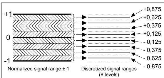
Fig. 14: Discrete values assignment for 8 quantization intervals
