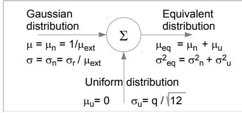
Fig. 10: PQN model for evaluation of quantization noise effects.
