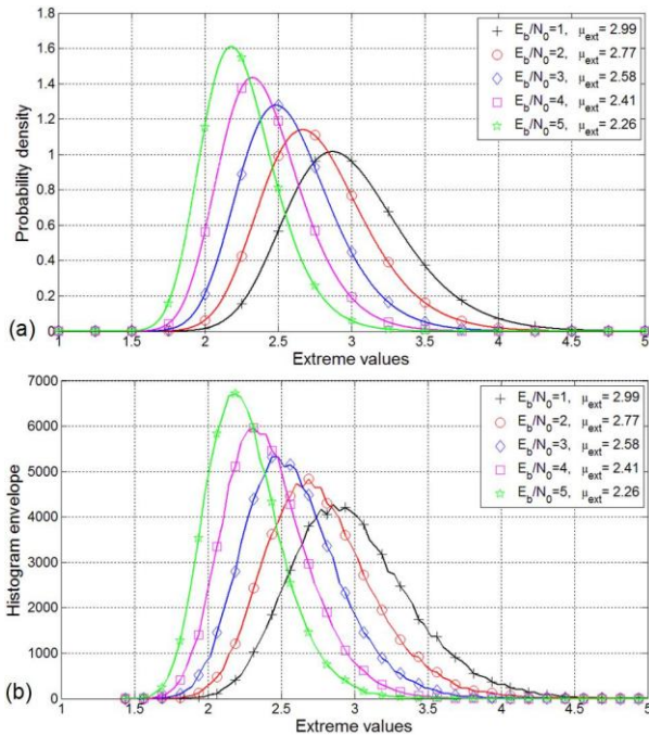
Fig. 9. (a) Theoretical extreme values distribution for C(48,24,12) and (b) corresponding simulation histograms.
