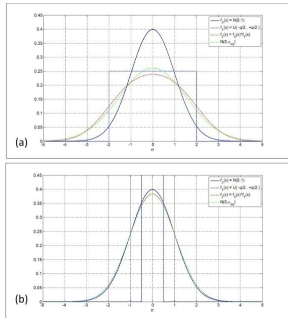
Fig. 12: Convolution of signal and quantization noise for (a) \alpha = 4 (b) \alpha = 1 .
