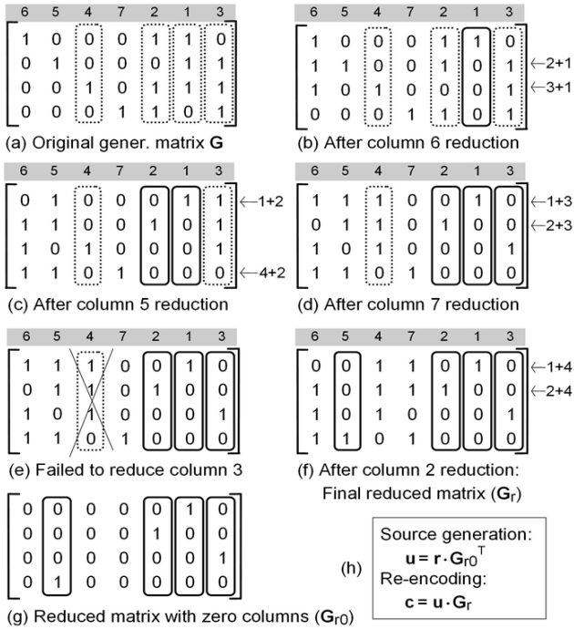
Fig. 1. Construction of the \mathbf{G}_r and \mathbf{G}_{r0} matrices.
