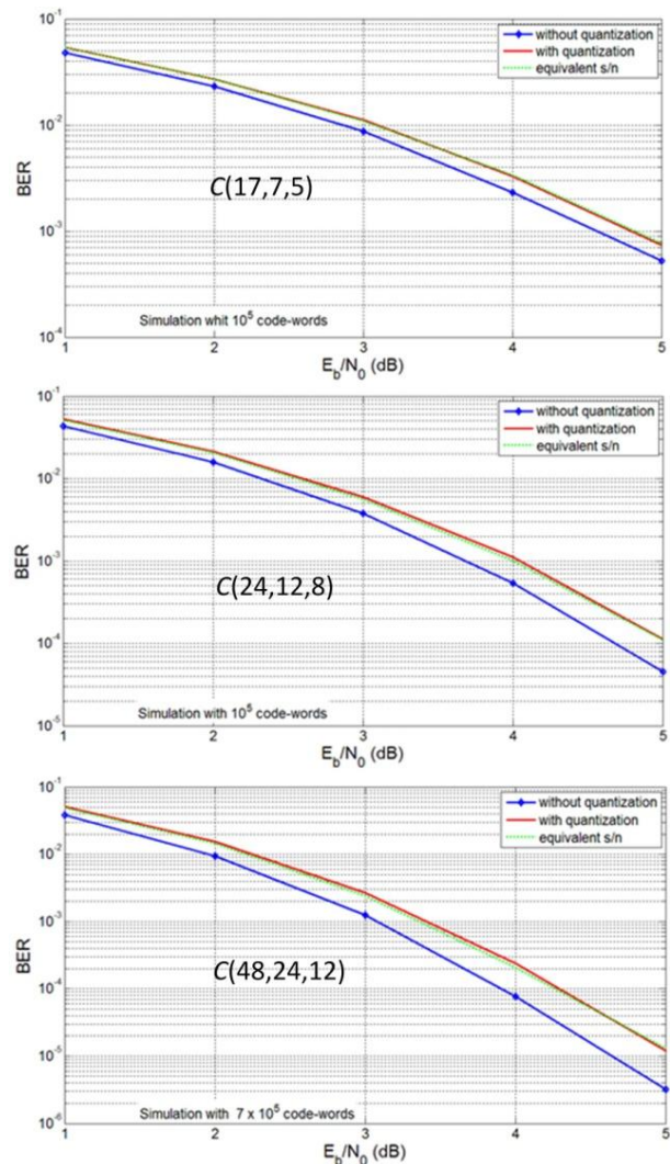
Fig. 15: Validation of the quantization effects (8 intervals) for several codes.
