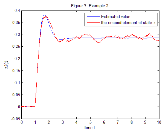
Fig. 3: Simulation result: true state (the second element of state x) and estimated value
