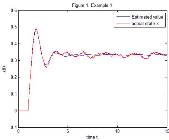
Fig. 1: Simulation result : true state and estimated value
