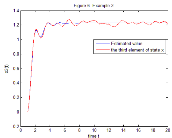
Fig. 6: Simulation result: true state (the third element of state x) and estimated value
