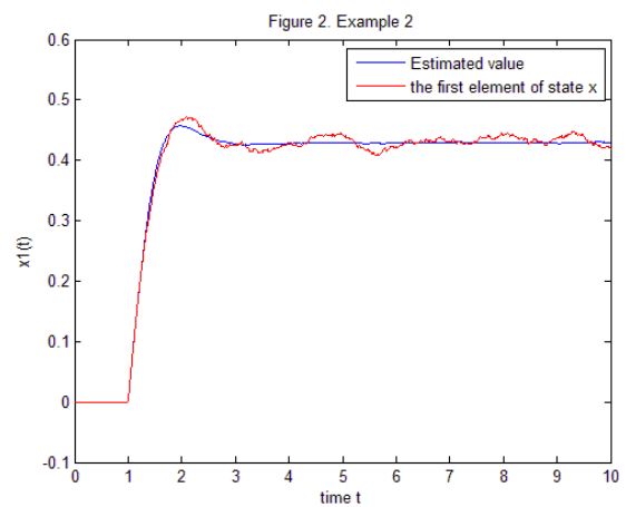
Fig. 2: Simulation result: true state (the first element of state x) and estimated value
