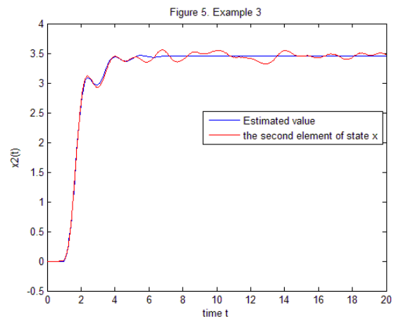
Fig. 5: Simulation result: true state (the second element of state x) and estimated value
