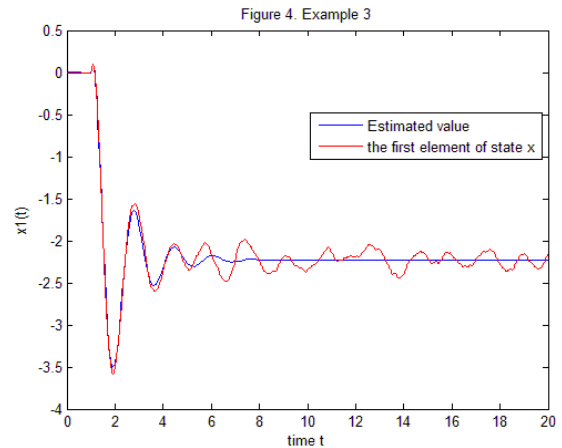
Fig. 4: Simulation result: true state (the first element of state x) and estimated value
