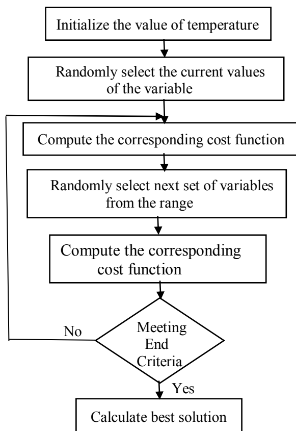
Fig. 3 Flow Chart of SAA
