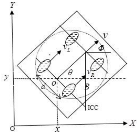
Fig.1 (a) Four wheeled Mobile Robot Configuration
