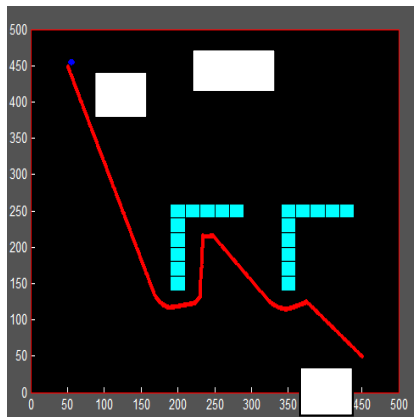
Fig. 6 (a) Robot Start Point (450, 50), Target (50,450)
