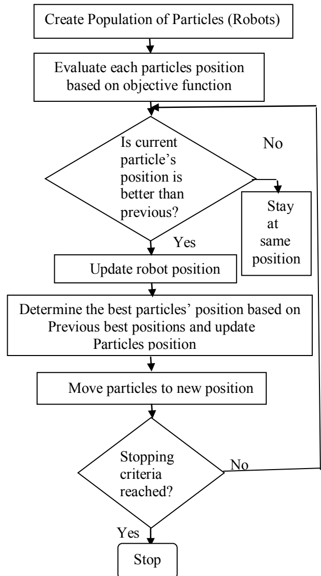
Fig. 5 Flow Chart of PSO Algorithm
