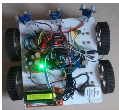
Fig.9 (a) Mobile Robot set up
