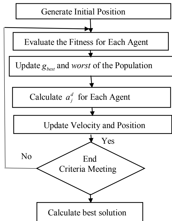
Fig.2 Flow Chart of GSA
