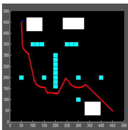
Fig. 7 (c) Robot Start Point (450, 50), Target (50,450)
