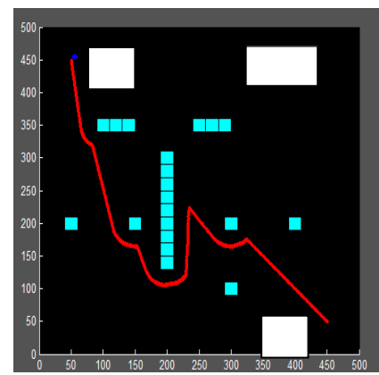
Fig. 7 (a) Robot Start Point (450, 50), Target (50,450)
