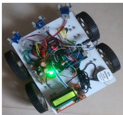
Fig.9 (b) Mobile Robot with GPS Antenna, Magnetic compass and LCD Unit
