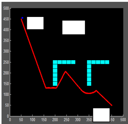
Fig. 6 (b) Robot Start Point (450, 50), Target (50,450)
