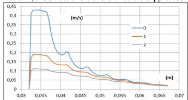
Fig. 14 Velocity suppressing at the frontal side of the bobbin by blinding of 0-1-2 rows of orifices in the perforated core
