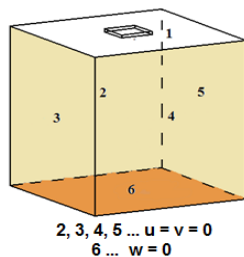
Fig. 6 Boundary conditions
