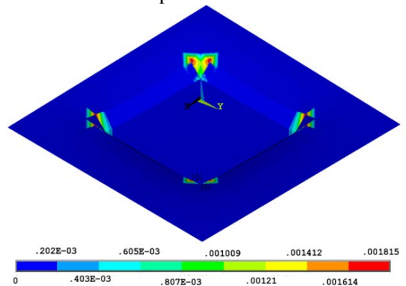
Fig. 11 Plastic deformations [m]
