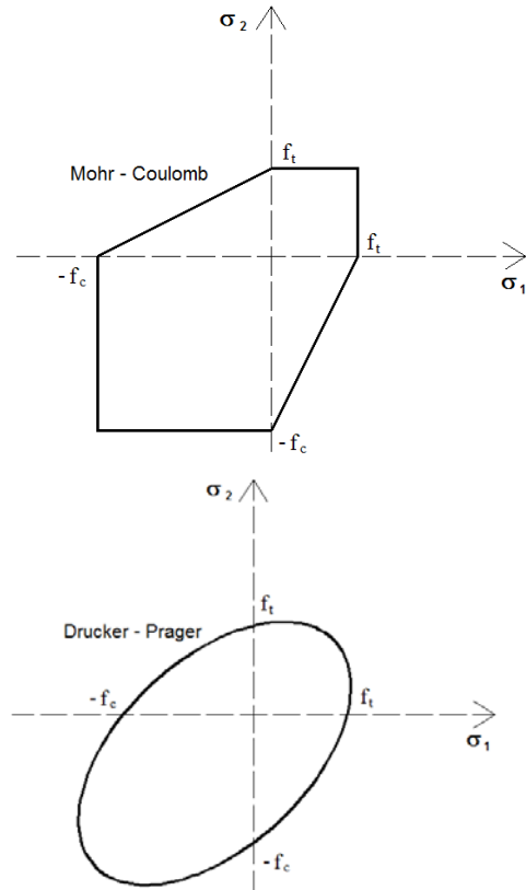
Fig. 3 Mohr - Coulomb and Drucker-Prager condition of plasticity, sectional view for plane stress
