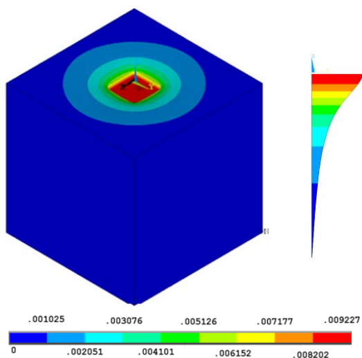
Fig. 10 Total deflection; vertical section in subsoil [m]
