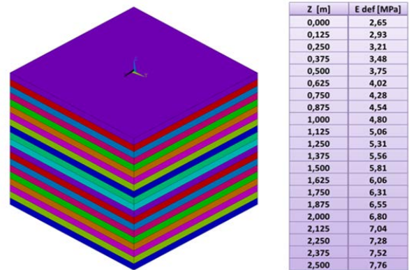
Fig. 7 Layers of the inhomogeneous half-space
