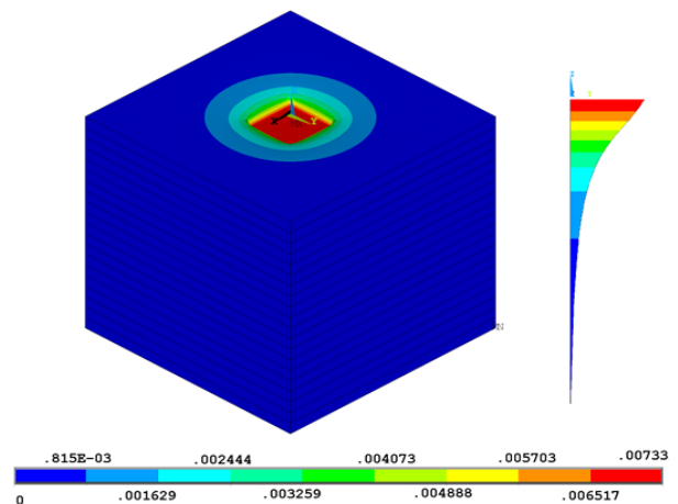
Fig. 8 Total deflection; vertical section in subsoil [m]
