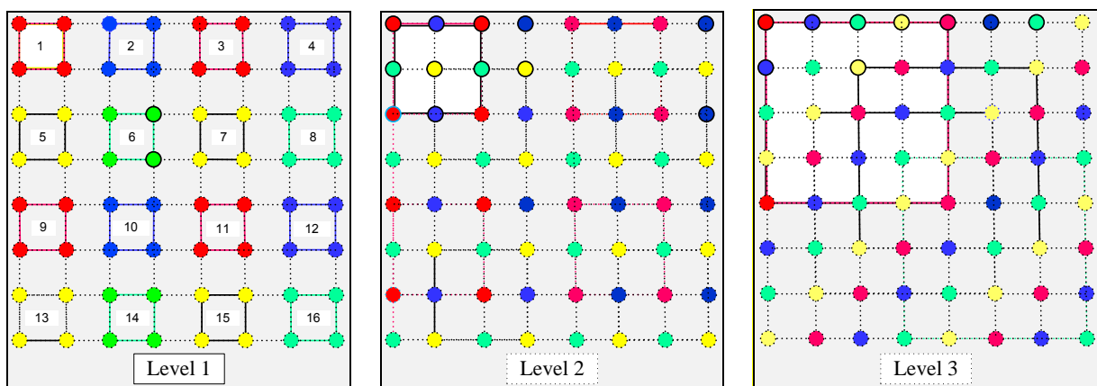
Fig.7. Section for tensor of size 8x8x8 in levels 1, 2, and 3 of the 3-level HSVD 8x8x8 algorithm, based on the SVD 2x2 (each tensor here is represented as a matrix of size 8x8; in each level, the SVD 2x2 is executed 16 times)
