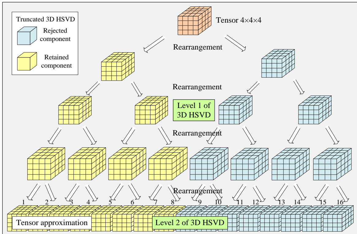
Fig.6. Structure of the computational graphs of the full and truncated 4-level binary tree for the execution of the 2-level 3D HSVD 4x4x4 algorithm based on the SVD 2x2
