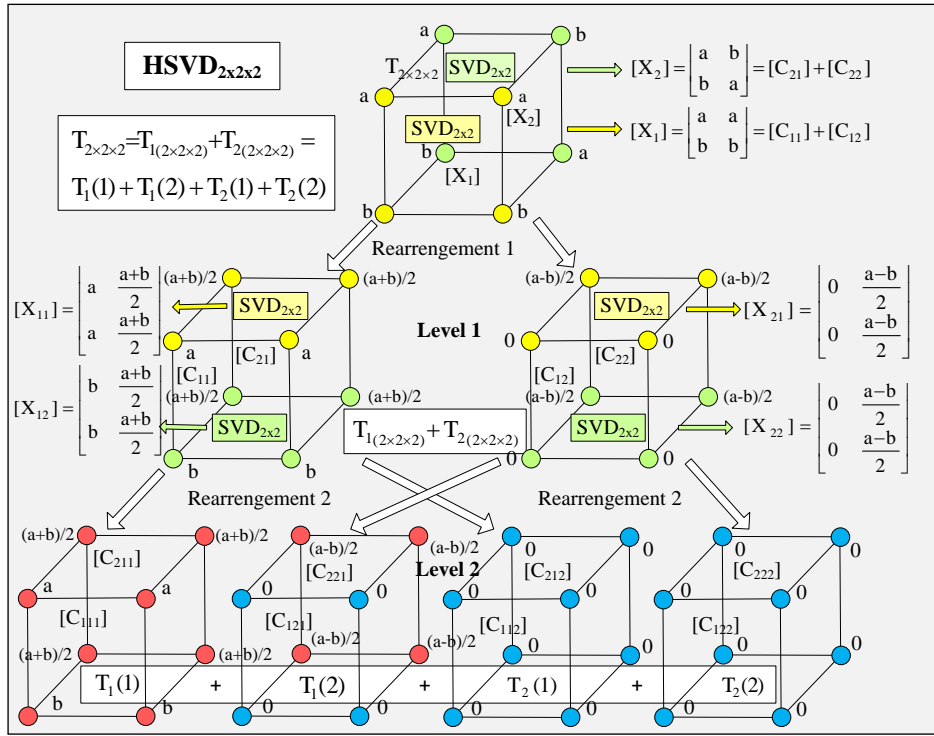
Fig. 8. Example: two-level HSVD 2x2x2 for elementary tensor T 2x2x2
