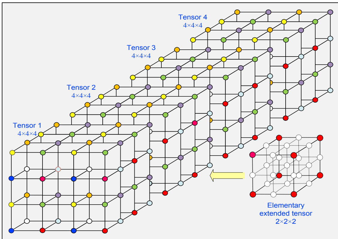
Fig. 5. Division of tensors T_{i(4 \times 4 \times 4)}(j) into the elementary tensors T_{j(2 \times 2 \times 2)}(i) in the second HSVD_{4 \times 4 \times 4} level, where the HSVD_{2 \times 2 \times 2} is applied on each group of voxels of same color (32 in total)
