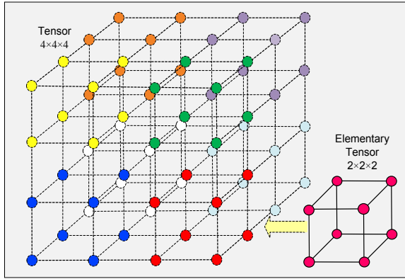
Fig. 4. The tensor T_{4 \times 4 \times 4} is divided into eight elementary tensors T_{2 \times 2 \times 2}(i) for i=1,2,\dots,8 in the first HSVD_{4 \times 4 \times 4} level, where the HSVD_{2 \times 2 \times 2} is applied on each group of voxels of same color (8 in total)
