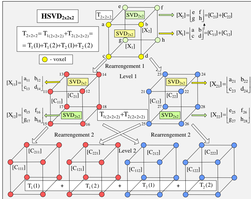
Fig. 2. Two-level HSVD 2x2x2 algorithm for elementary tensor of size 2x2x2 based on the SVD 2x2
