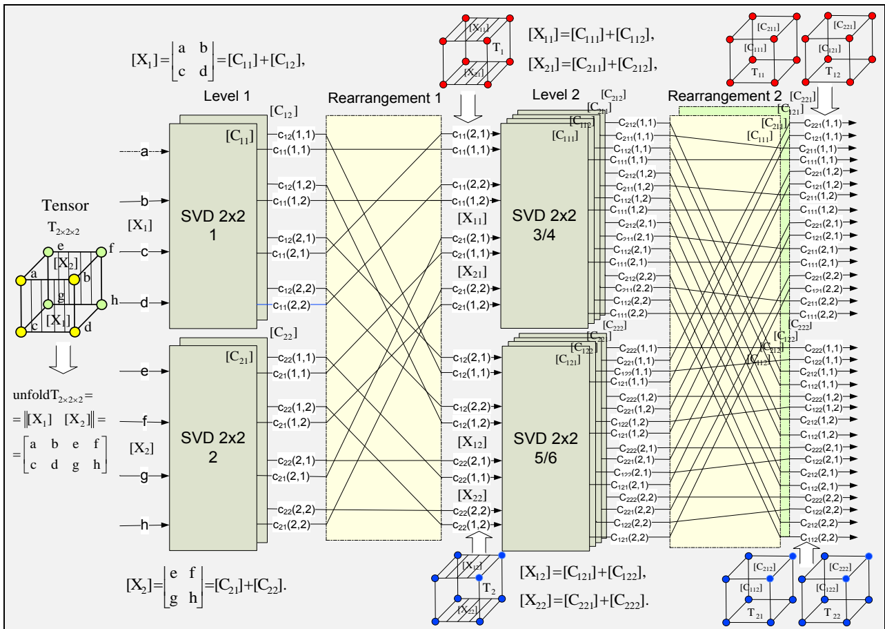
Fig. 3. The flow graph of the 2-level HSVD for the elementary tensor T_{2 \times 2 \times 2} , based on the SVD 2x2
