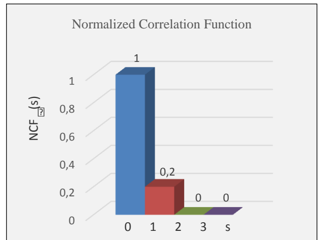
Fig. 9. The Normalized Correlation Function of the decomposition components
