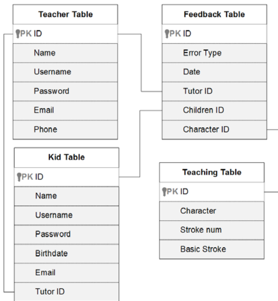
Figure 6. AHCE database
